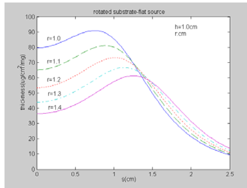
Fig.2. Theoretical film thickness distributions for a source-to-substrate distance h=1.0\text{cm} .
