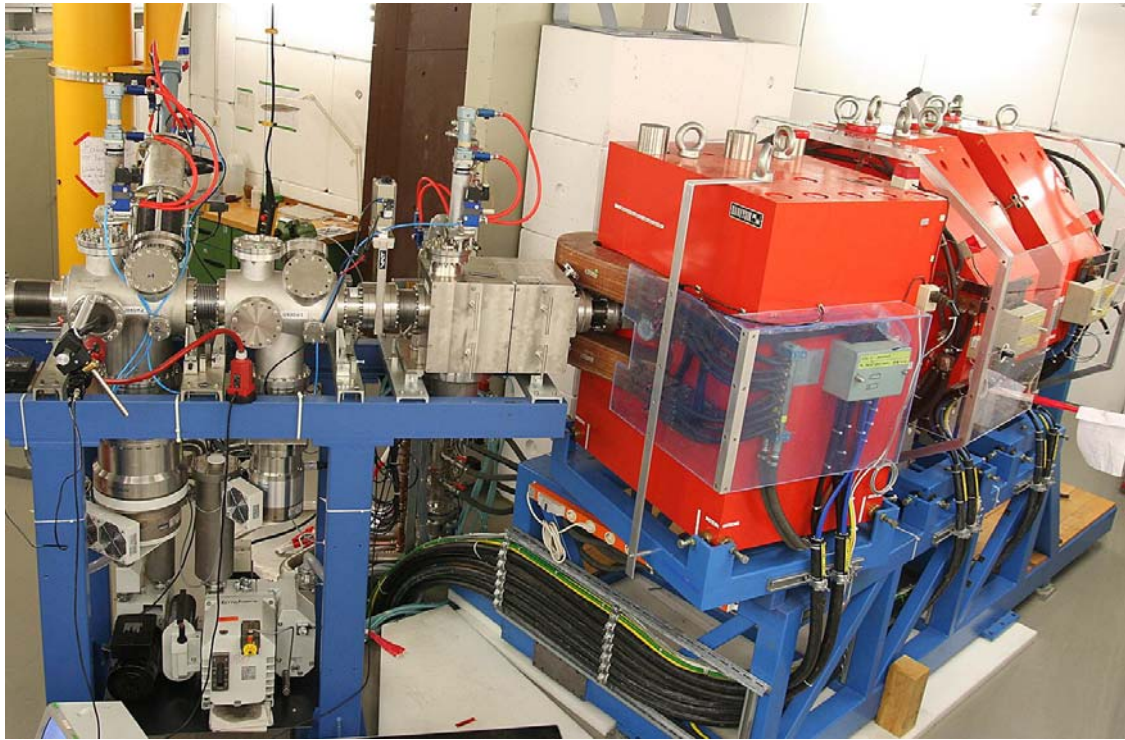
Fig. 2: View (from left to right, beam direction) of two diagnosis chambers, the target chamber (center) and the TASCA magnets.
