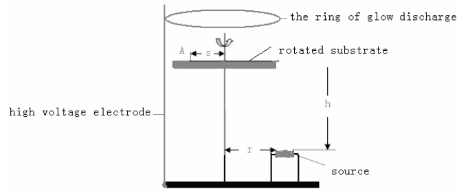
Fig.1.Schematic drawing of the rotating substrate set-up.
